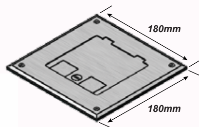
145 (IP55) Square Lid Section (Bevelled Edge)
