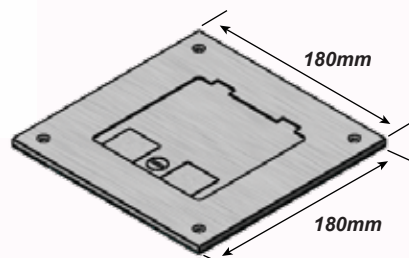
145 (IP55) Square Lid Section (Square Edge)
