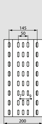
Width 200 mm
