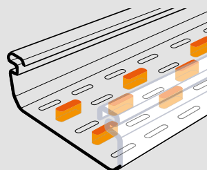
9 x 25 mm perforations for PVC screws - diameter 8 mm
