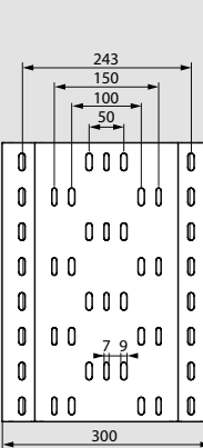
Width 300 mm
