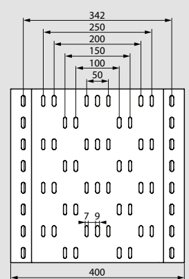
Width 400 mm
