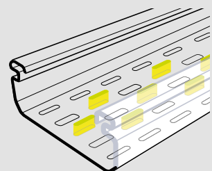
7 x 25 mm perforations for PVC screws - diameter 6 mm
