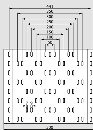
Width 500 mm
