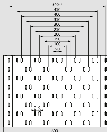
Width 600 mm
